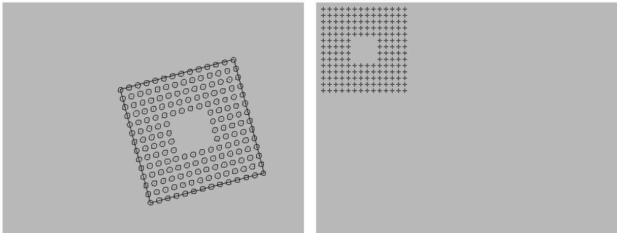
Figure 4.25: Normalization of the grid for the reference BGA: (left) smallest rectangle enclosing the region that is built by the center points of the balls, (right) transformed and normalized grid (scaled for visualization purposes).
