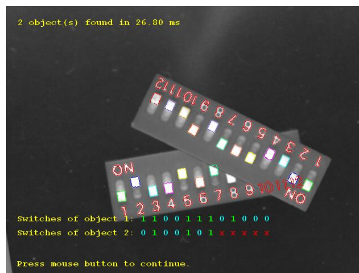
Figure 3.35: Result of component-based matching: two instances of a component model showing a dip switch are found, although some components are occluded.
