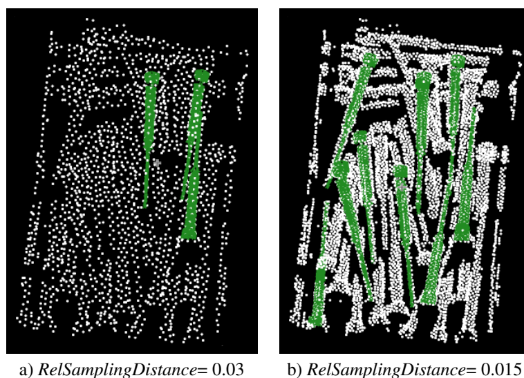
Figure 5.1: With the determined distance between the sampling points of a scene, the object characteristics still need to be represented.
